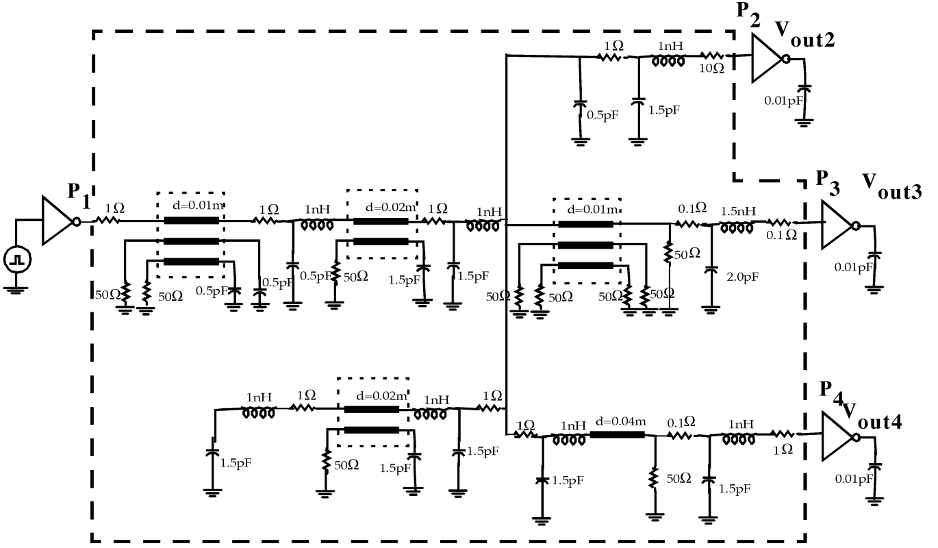
Fig. 10. Four-port interconnect subnetwork (example 2).
